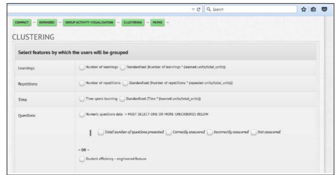
Figure 10 On demand clustering – feature selection
